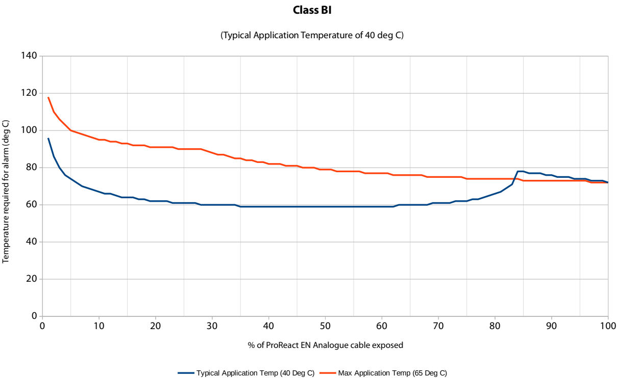
Chart 2 - Expected temperature required for an alarm in relation to percentage of ProReact EN Analogue LHD Cable in Class BI Setting
